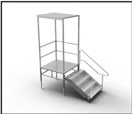
4 STEP STAIR WITH CANOPY
